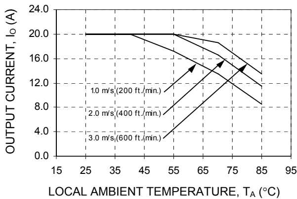
Figure 16. Output Current Derating for the QBK020A0B ( V_o = 12V ) in the Transverse Orientation with baseplate and 0.25-inch high heatsink; Airflow Direction from V_{in}(+) to V_{in}(-) ; V_{in} = 48V .
