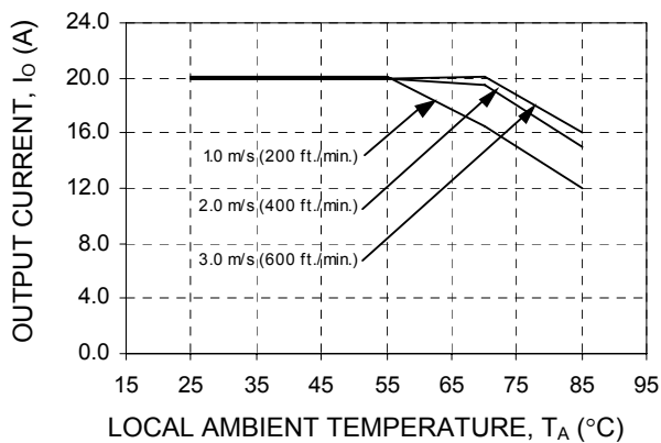
Figure 17. Output Current Derating for the QBK020A0B ( V_o = 12V ) in the Transverse Orientation with baseplate and 0.5-inch high heatsink; Airflow Direction from V_{in}(+) to V_{in}(-) ; V_{in} = 48V .
