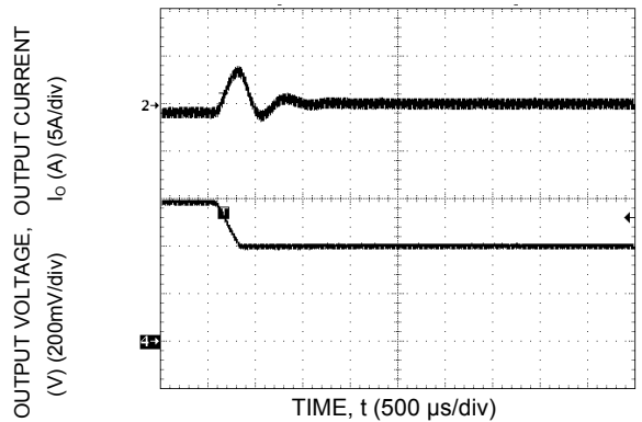
Figure 6. Typical Transient Response to Step Change in Load from 75% to 50% of Full Load at Room Temperature and 48 Vdc Input.
