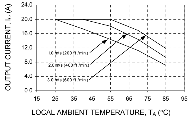
Figure 15. Output Current Derating for the QBK020A0B ( V_o = 12 V) in the Transverse Orientation with baseplate; Airflow Direction from V_{in}(+) to V_{in}(-) ; V_{in} = 48 V.
