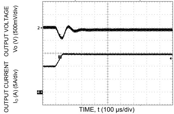
Figure 5. Typical Transient Response to Step change in Load from 50% to 75% of Full Load at Room Temperature and 48 Vdc Input.
