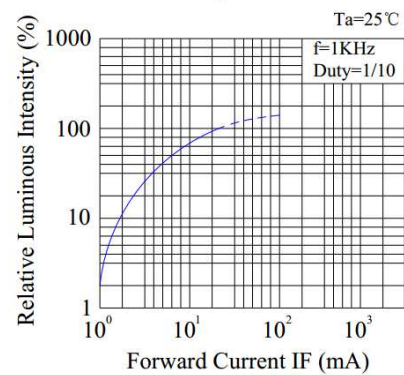
Luminous Intensity & Forward Current T_a=25^\circ\text{C}
