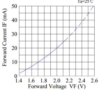
Forward Current & Forward Voltage T_a=25^\circ\text{C}
