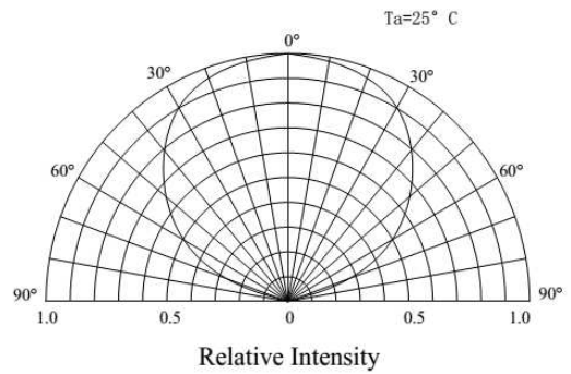
RADIATION PATTERN
