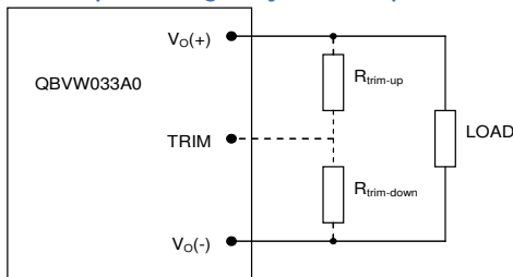
Figure 16. Circuit Configuration to Trim Output Voltage.
