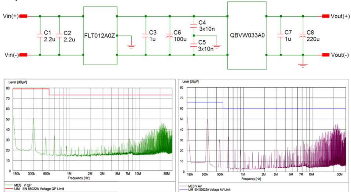
Figure 26. EMC Considerations
