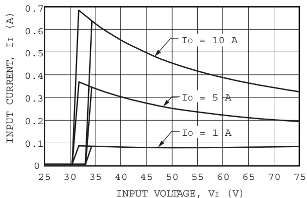
Figure 1. Typical QHW050Y1 Input Characteristics at Room Temperature
