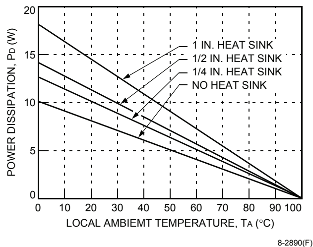
Figure 33. Heat Sink Power Derating Curves; Natural Convection; Longitudinal Orientation
