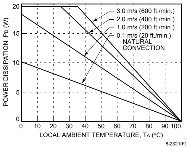
Figure 25. Forced Convection Power Derating with No Heat Sink; Transverse Orientation
