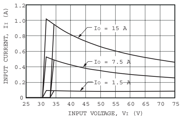
Figure 2. Typical QHW075Y1 Input Characteristics at Room Temperature
