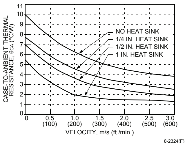
Figure 31. Case-to-Ambient Thermal Resistance Curves; Longitudinal Orientation
