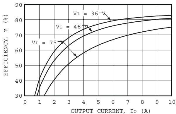
Figure 4. Typical QHW050Y1 Converter Efficiency vs. Output Current at Room Temperature
