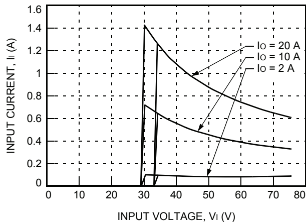
Figure 3. Typical QHW100Y1 Input Characteristics at Room Temperature
