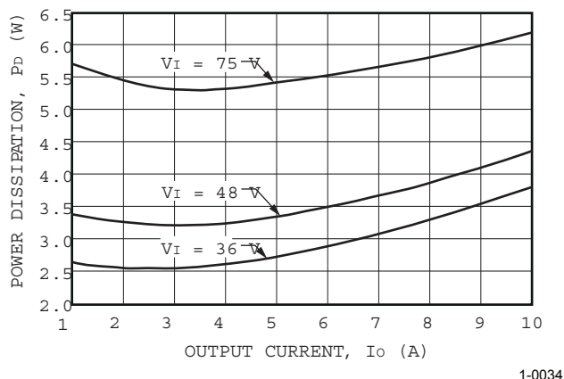
Figure 27. QHW050Y1 Power Dissipation vs. Output Current at 25 °C
