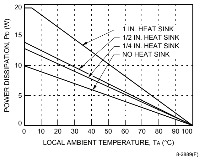
Figure 32. Heat Sink Power Derating Curves; Natural Convection; Transverse Orientation
