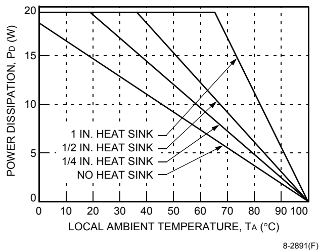
Figure 34. Heat Sink Power Derating Curves; 1.0 m/s (200 lfm); Transverse Orientation
