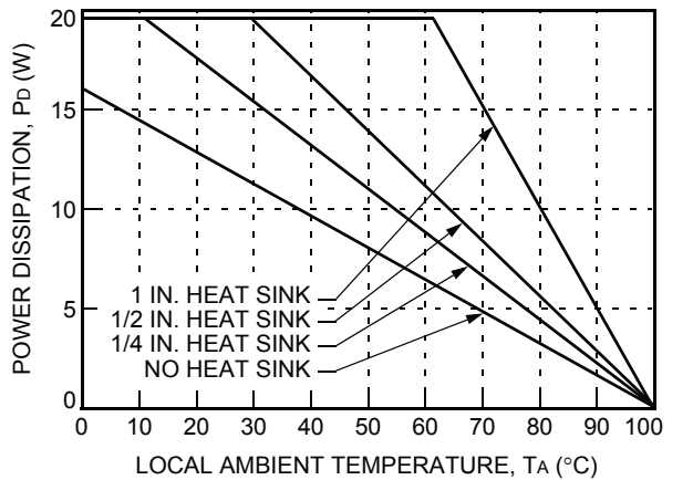
Figure 35. Heat Sink Power Derating Curves; 1.0 m/s (200 lfm); Longitudinal Orientation
