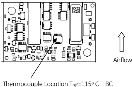
Figure 14. T_{ref} Temperature measurement location.
