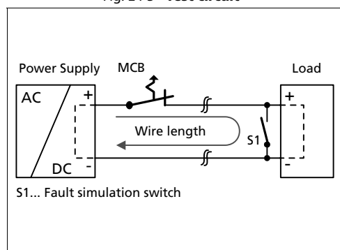
Fig. 24-3 Test circuit
