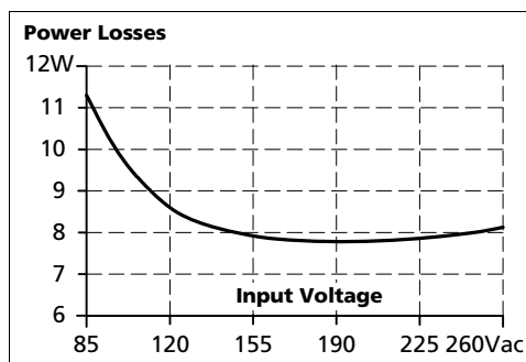
Fig. 9-4 Losses vs. input voltage at 3.8A, typ.
