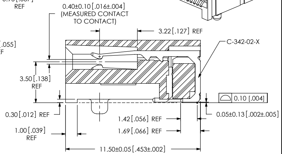
FIG 1 QSFP8-038-01-X-D-RA1 SHOWN
