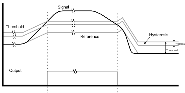
Figure 2-1 Drift Compensation
