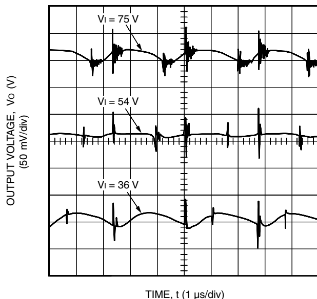
Figure 5. Typical QW050A1 Output Ripple Voltage at Room Temperature and I_o = I_{o, \text{max}}
