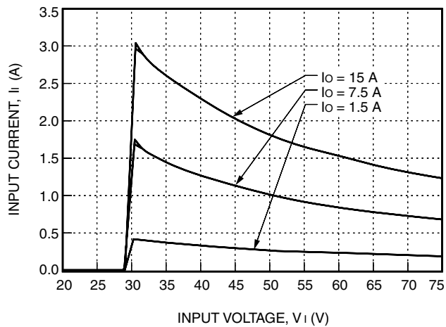
Figure 2. Typical QW075A1 Input Characteristics at Room Temperature
