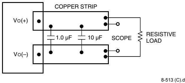
Figure 13. Input Reflected-Ripple Test Setup
