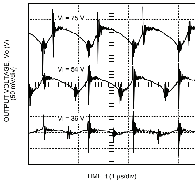
Figure 6. Typical QW075F1 Output Ripple Voltage at Room Temperature and 10 A Output
