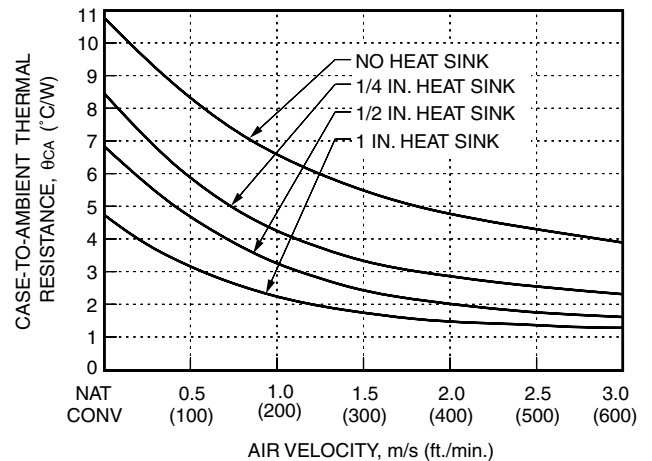
Figure 26. Case-to-Ambient Thermal Resistance Curves; Transverse Orientation
