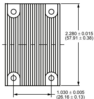
Figure 33. Longitudinal Heat Sink
