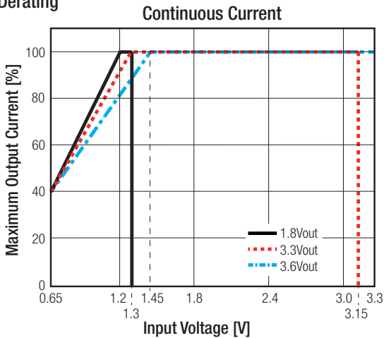
Line Derating
