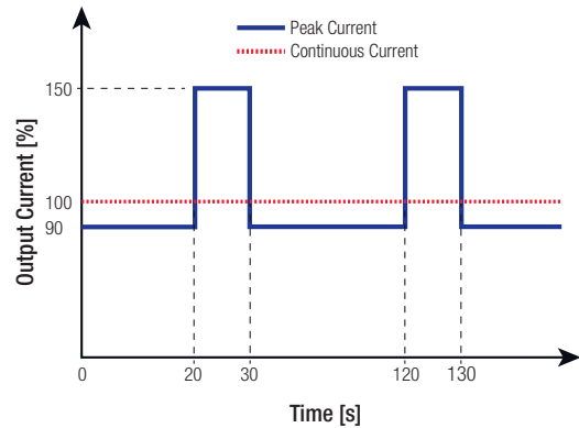
Overload Capability
