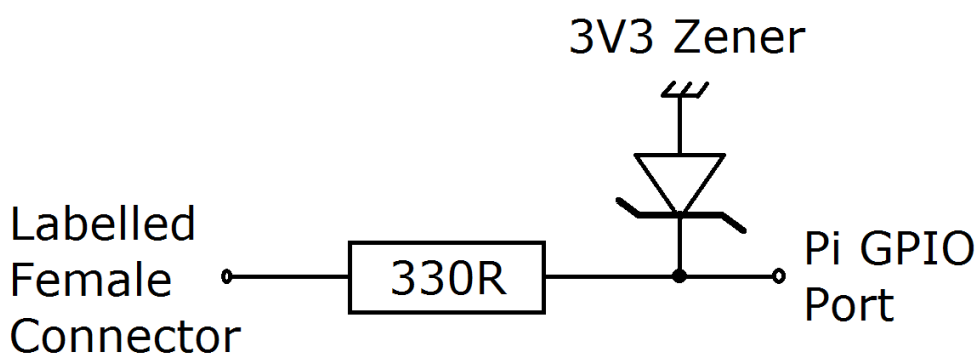
Schematic of port protection circuit
