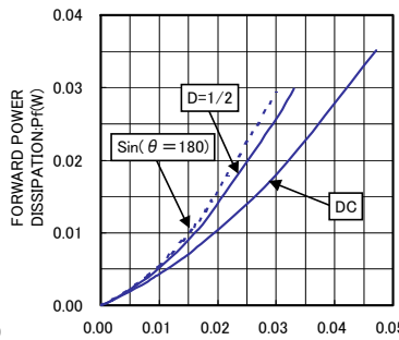
Io-Pf CHARACTERISTICS
