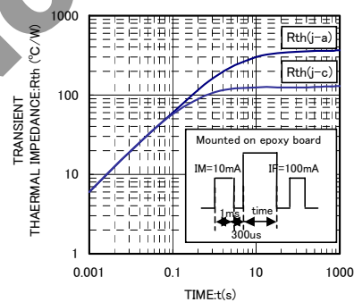
Rth-t CHARACTERISTICS
