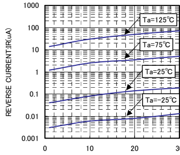
VR-IR CHARACTERISTICS
