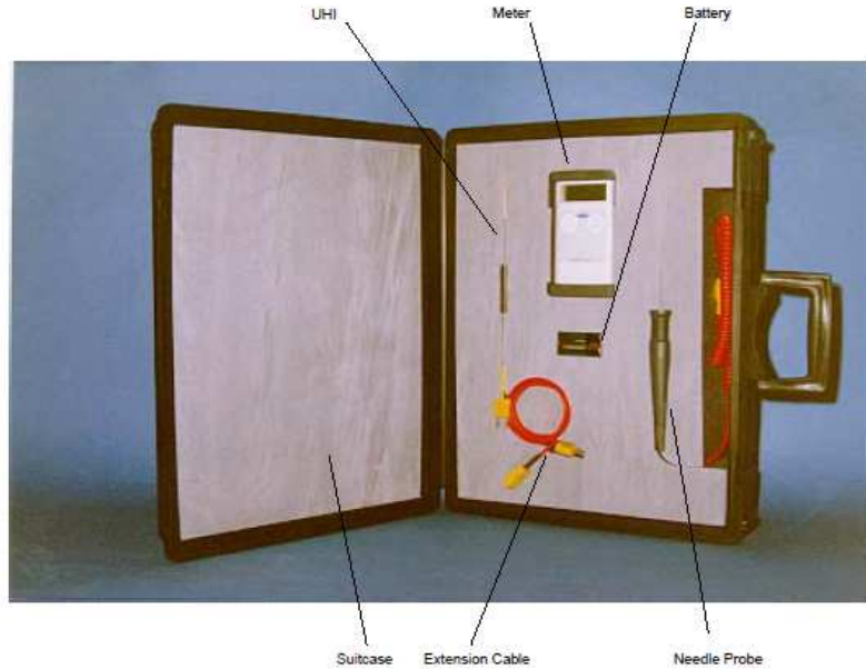
Temperature calibration kit in a case containing meter, UHI probe + cable & needle probe
