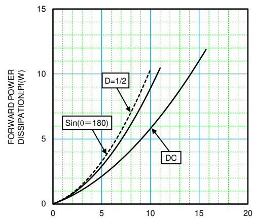
AVERAGE RECTIFIED FORWARD CURRENT : I_o (A) I_o - P_i CHARACTERISTICS
