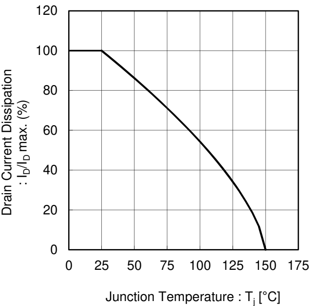
Fig.17 Drain Current Derating Curve
