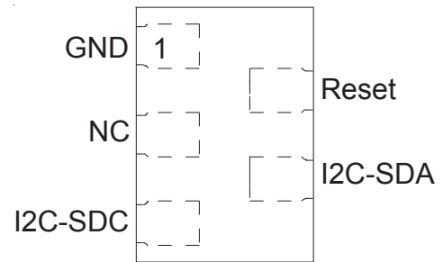
Figure 2 - Pin Configuration (Top View) for Camera Data Line Protection Applications
