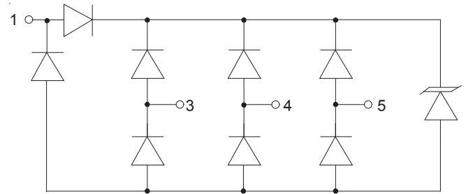
Figure 1 - Circuit Diagram
