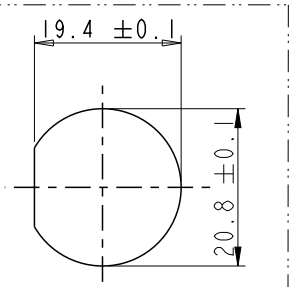
Recommended Panel Cut-Out Rear View
