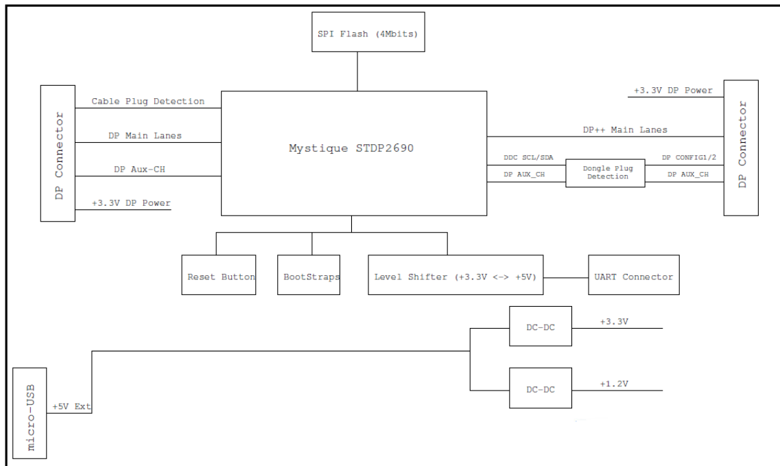
Figure 2. Connection diagram
