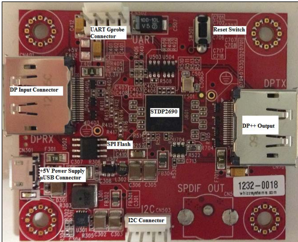
Figure 3. Board picture
