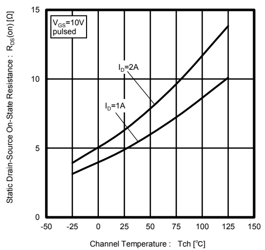
Fig.6 Static Drain-Source On-State Resistance vs. Channel Temperature
