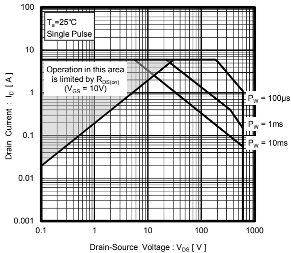
Fig.15 Maximum Safe Operating Area
