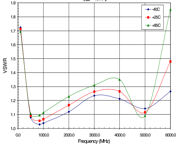
Input VSWR versus Frequency Across Temperature ( I_{CC} = 40\text{mA} )
