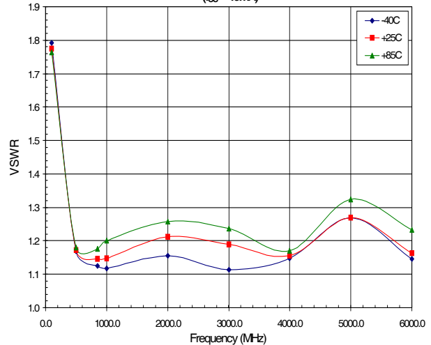
Output VSWR versus Frequency Across Temperature ( I_{CC} = 40\text{mA} )
