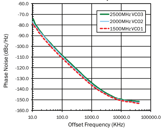
VCO Phase Noise With LO Divide by 2
