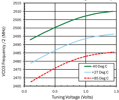
VCO3 Frequency versus Tuning Voltage For the same coarse tune setting, LO divide by two
