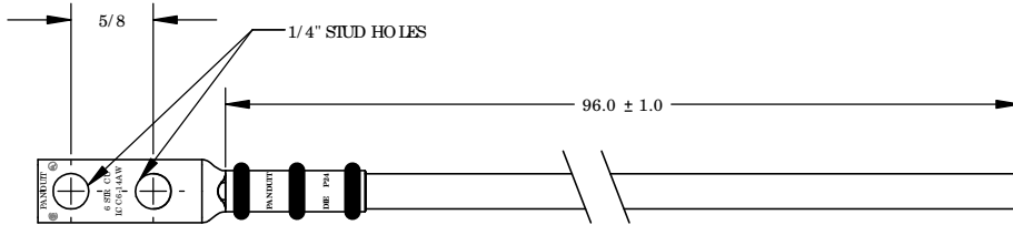
FACTORY CRIMPED # 6 AWG/16mm SQ. COMMON BONDING NETWORK (CBN) JUMPER WIRE ASSEMBLY (QTY. 1) INCLUDES: ICC6-14AW (QTY. 1) # 6 AWG/16mm SQ. WIRE - GREEN/YELLOW INSULATION 96" LONG
