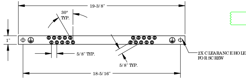
UNIVERSAL GROUND BAR - RGRB19U (QTY. 1) INCLUDES: - # 12-24 HEX HEAD SCREWS (QTY. 20) PRE-ASSEMBLED
