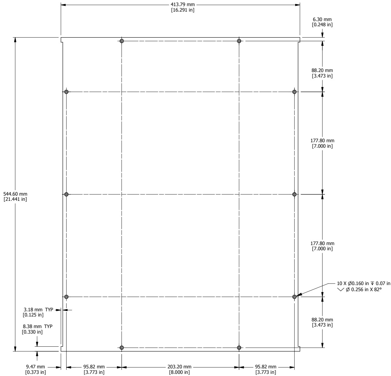
TOP VIEW
