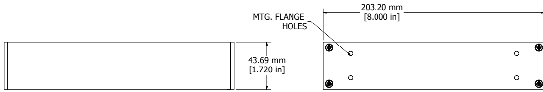
ASSEMBLY - VIEW FROM TOP
