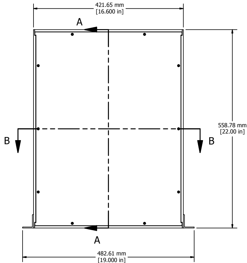
ASSEMBLY - TOP VIEW
