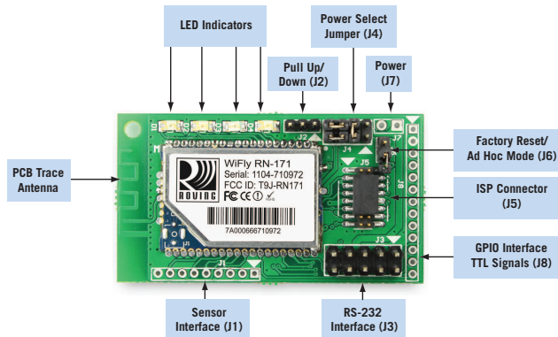
Figure 1. RN-174 Evaluation Board (Part 1 of 2)
