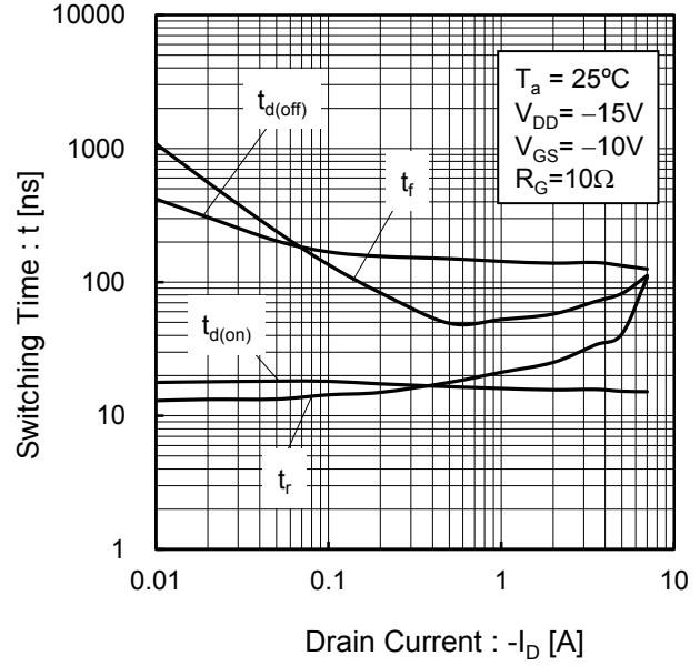
Fig.19 Switching Characteristics
