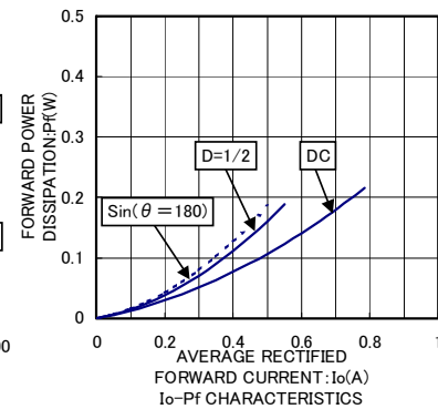
Io-Pf CHARACTERISTICS
