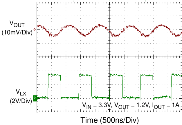
Voltage Ripple
