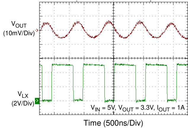
Voltage Ripple
