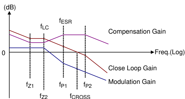
Figure 6. System Bode Plot
