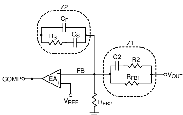
Figure 5. Type-III Compensator
