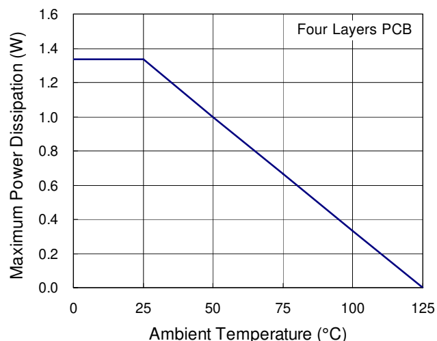
Figure 3. Derating Curve for RT8269 Package
