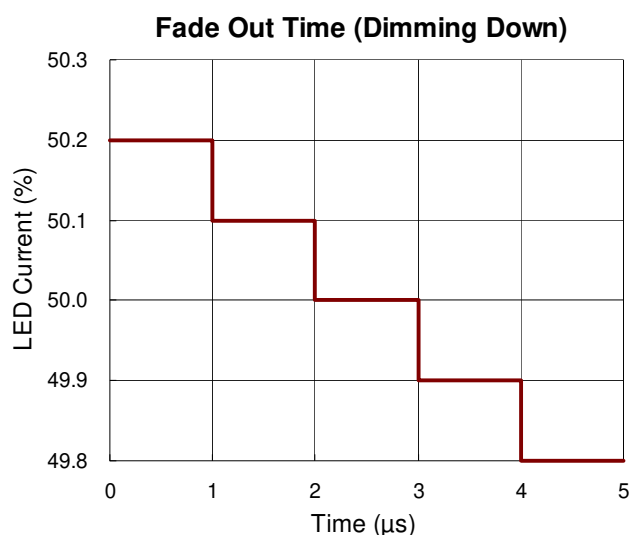
Figure 7. LED Current (Dimming Down) vs. Fade Out Time
