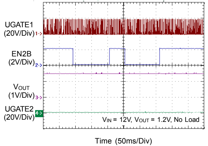
Single-phase Operation
