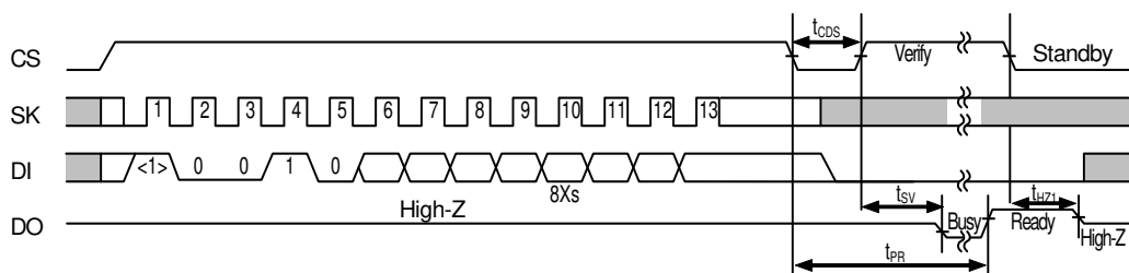
Figure 11 Chip Erase Timing
