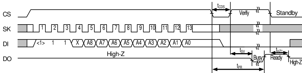
Figure 9 Data Erase Timing
