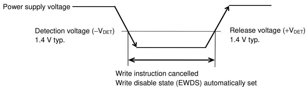
Figure 13 Operation during Low Power Supply Voltage
