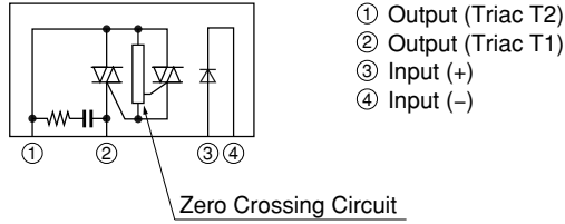
Zero Crossing Circuit
