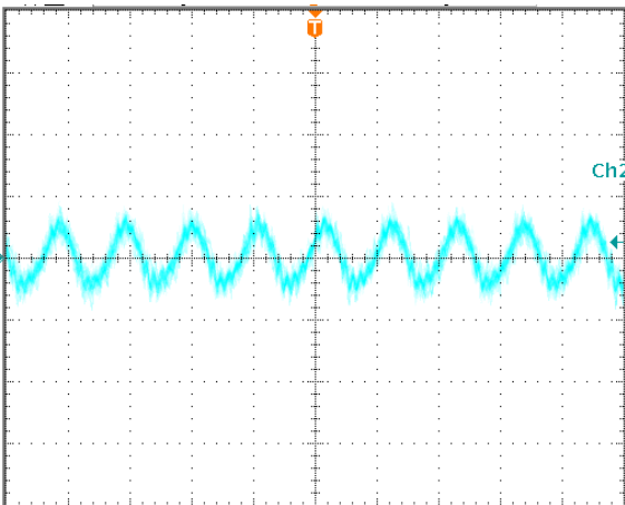
Output voltage ripple at nominal input voltage and max load current (4mV/div, 2us/div) Load cap: 10 \mu F, tantalum capacitor and 1 \mu F ceramic capacitor. Bandwidth: 20 MHz.
