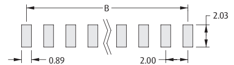
Recommended PC Board Pattern
