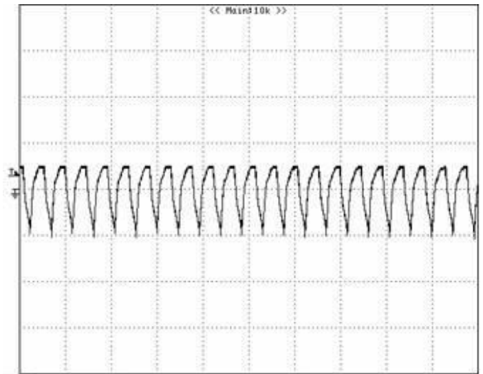
Figure 14: Output voltage ripple at nominal input voltage and rated load current ( I_o=2\text{A} )(50 mV/div, 5µs/div)
