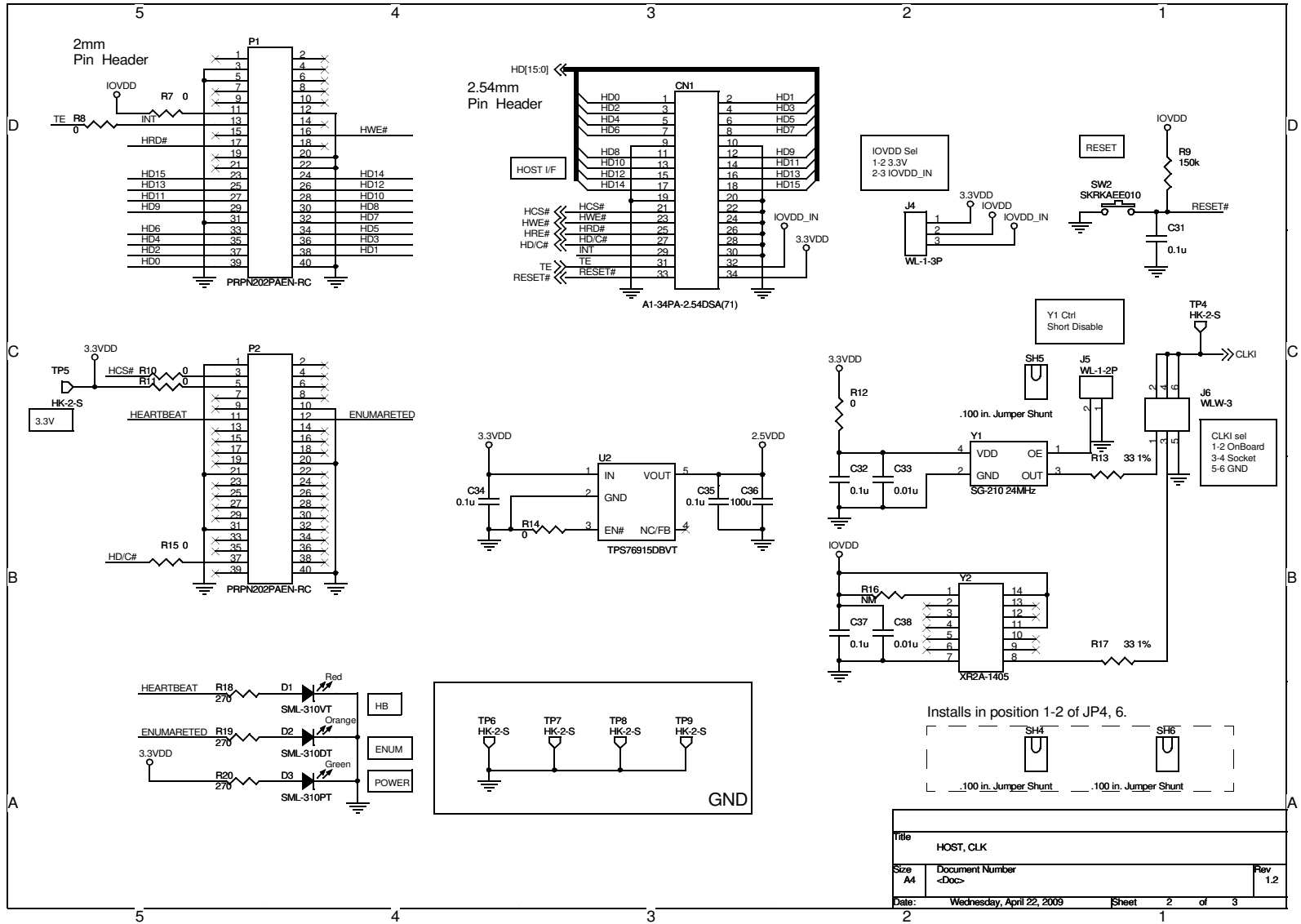
Figure 6-2: SSU13517P00C100 Schematic Diagram (2 of 3)
