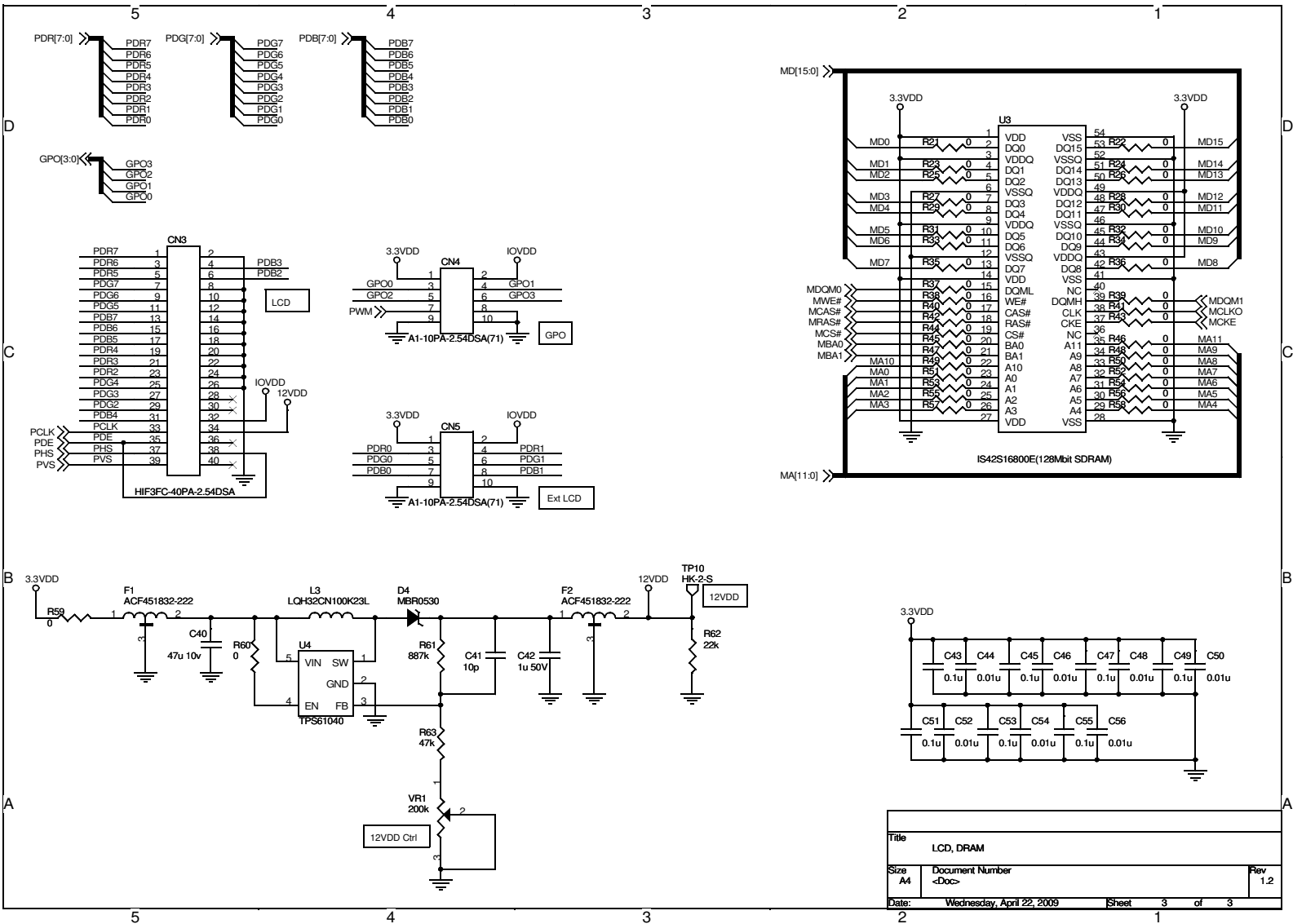
Figure 6-3: S5U13517P00C100 Schematic Diagram (3 of 3)
