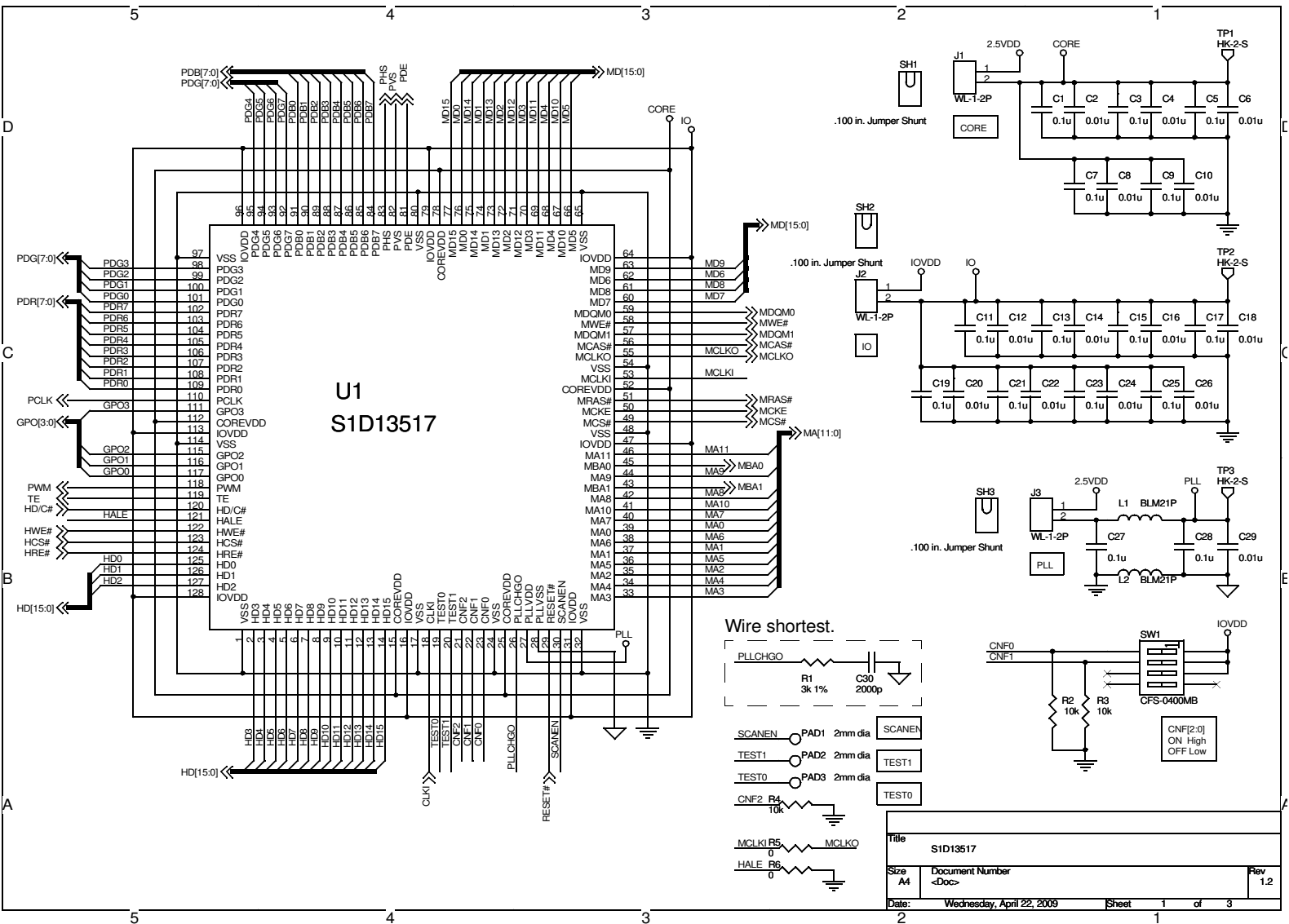
Figure 6-1: S5U13517P00C100 Schematic Diagram (1 of 3)
