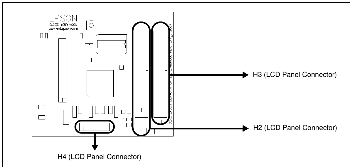
Figure 4-4: LCD Panel Connectors Location (H2, H3, H4)
