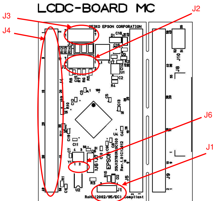
Figure 3-1 Jumper Pin Locations
