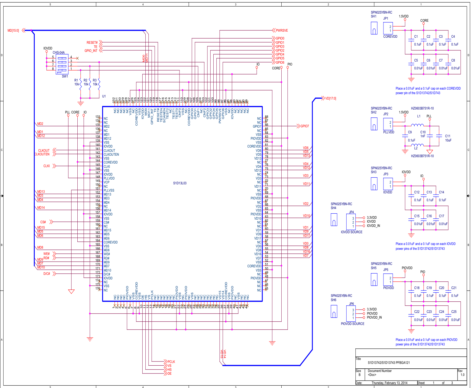
Figure 6-1: S5U13L03P00C100 Schematics (1 of 3)
