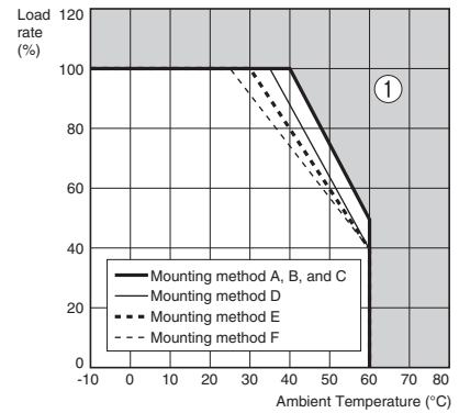
Models with Chassis and Cover (50W)
