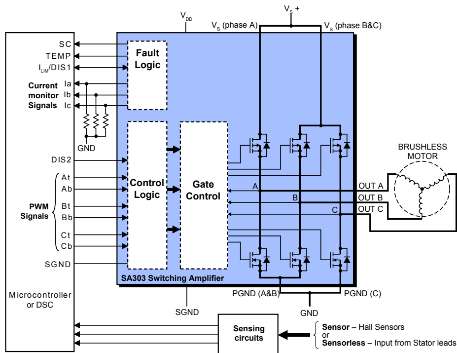
Figure 4. System Diagram
