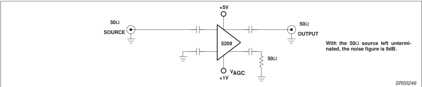
Figure 10. Underterminated Configuration
