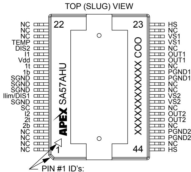
FIGURE 3. EXTERNAL CONNECTIONS - 44-Pin HSOP
