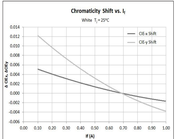
CIEx, y change as function of Current - White
