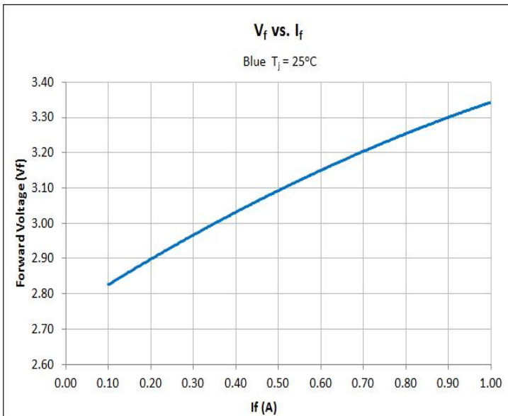
Voltage as function of Forward Current - Blue
