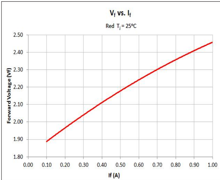
Voltage as function of Forward Current - Red
