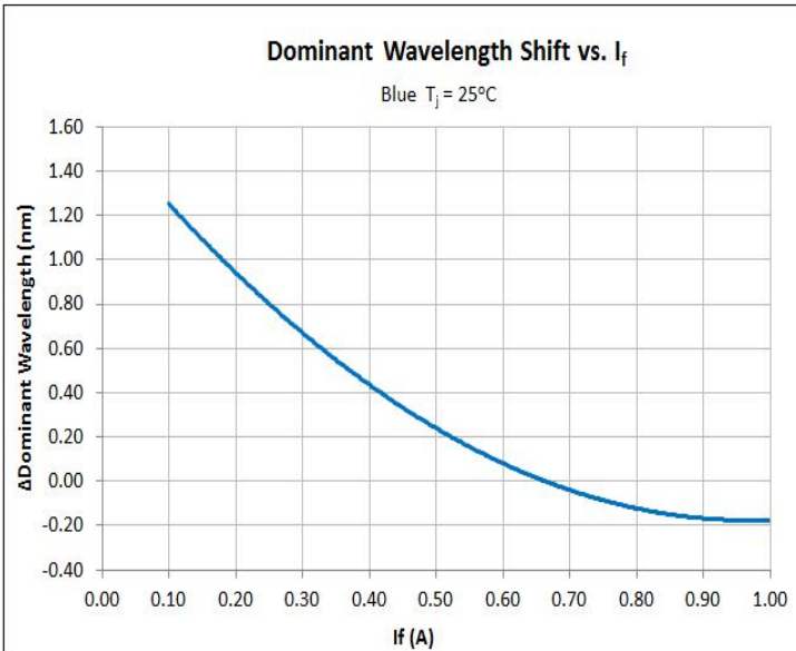
Wavelength change as function of Current - Blue
