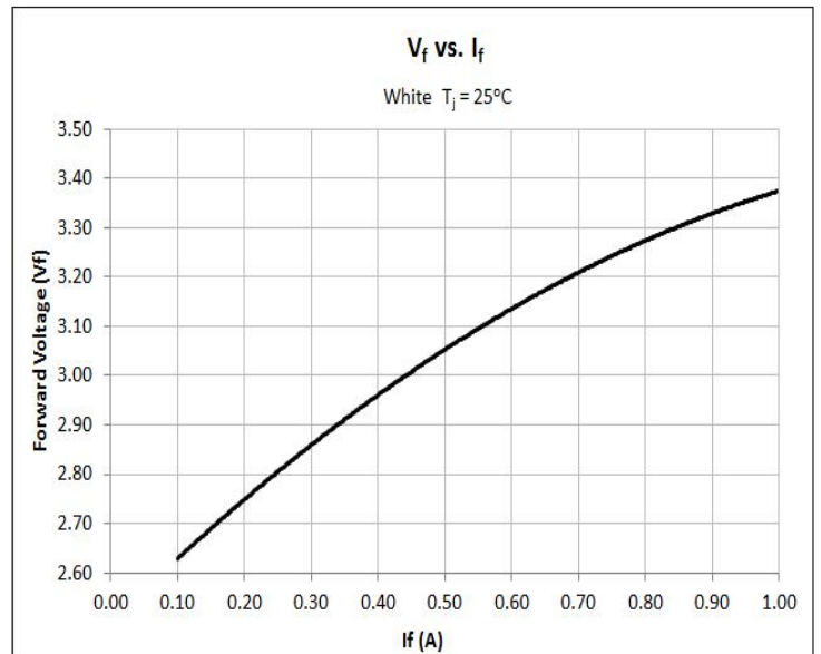
Voltage as function of Forward Current - White
