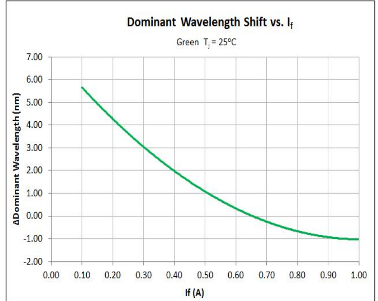
Wavelength change as function of Current - Green
