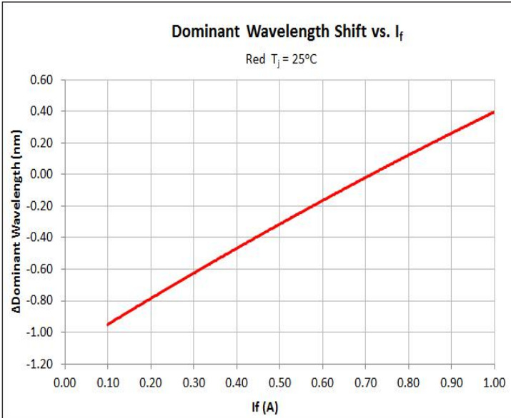
Wavelength change as function of Current - Red
