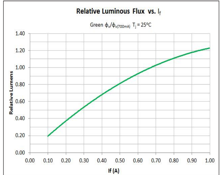
Relative Luminous Flux - Green
