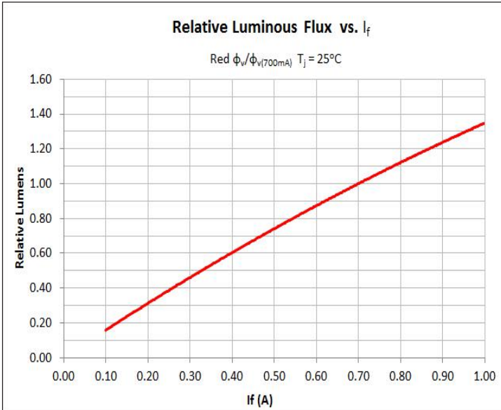
Relative Luminous Flux - Red
