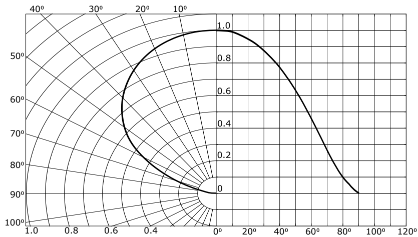
SBM-40-LC -RGBW Angular Distribution
