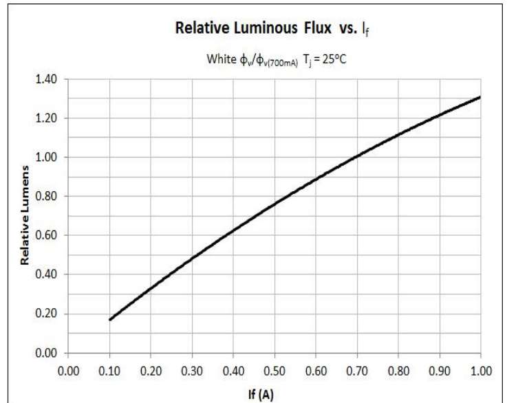
Relative Luminous Flux - White
