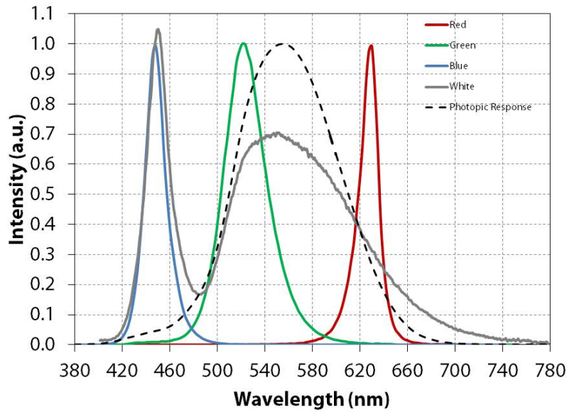
SBM-40-LC -RGBW Spectrum 8
