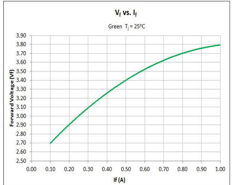
Voltage as function of Forward Current - Green
