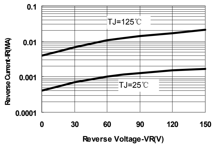
Fig.2-Typical Reverse Characteristics
